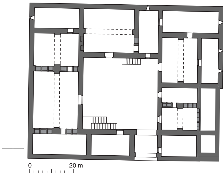
Fig. 4.2. Plan of the House of Flavius Seos in al-Ḥayyat. Drawing by Marion Berti, after Sartre-Fauriat 2004 (W. J. Banks).
